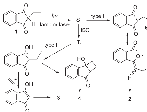
Scheme 2. Competing Norrish type I and type II mechanistic pathways.
